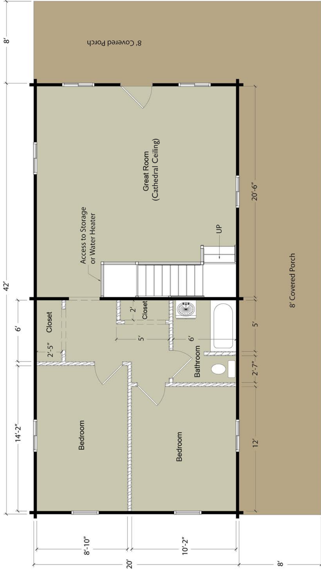
20' x 42' Custom Log Cabin - Reference 1C First Floor 840 Sq. Ft.
