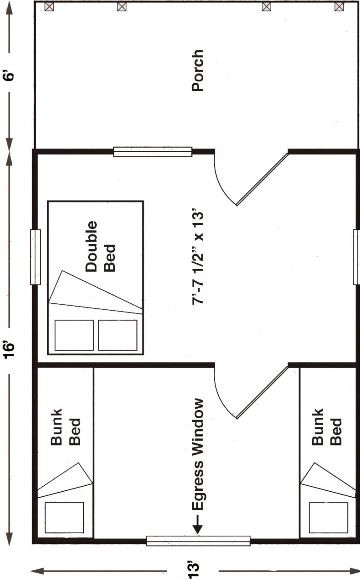
13' x 16' Timber Frame Cabin
