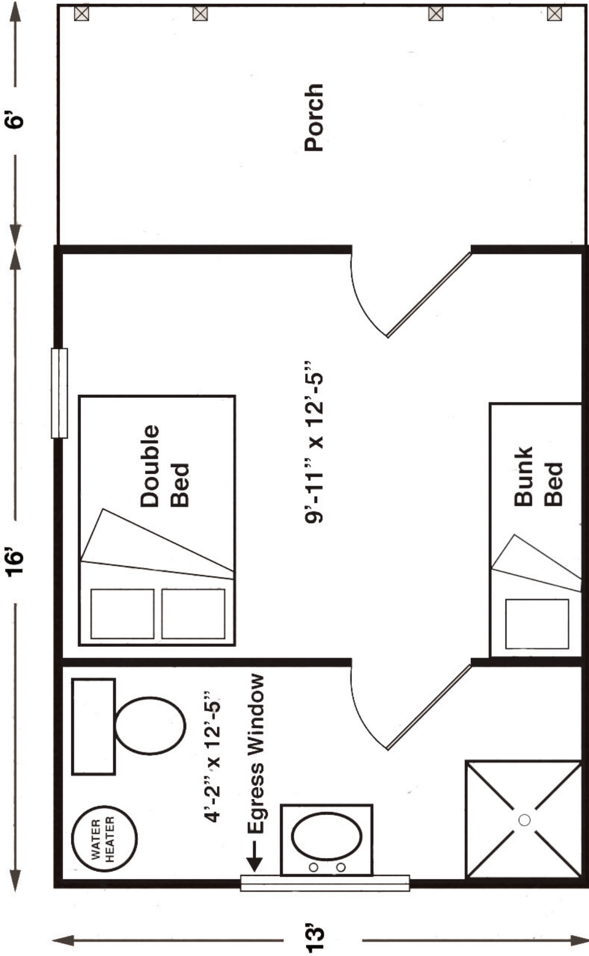
13' x 16' Timber Frame Cabin w/Bath
