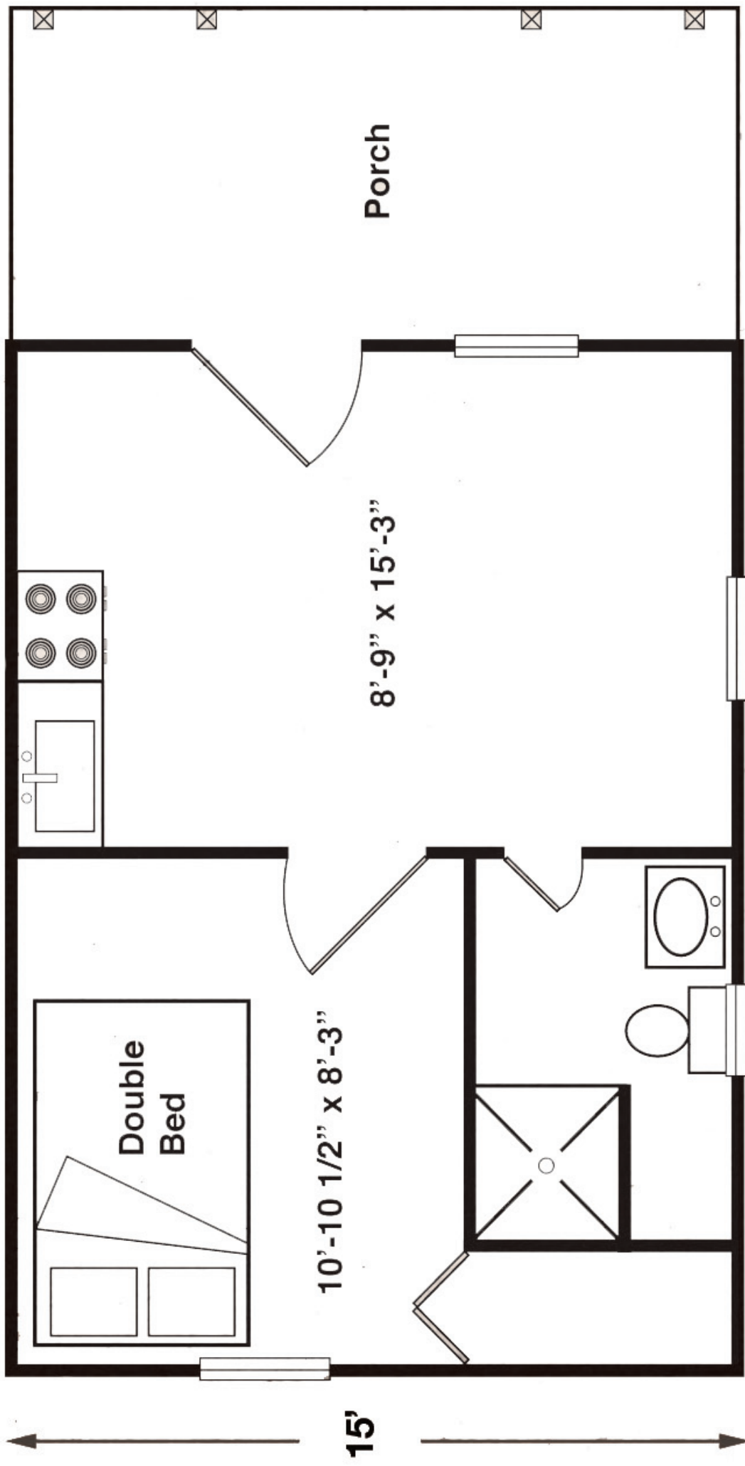
15' x 21' Timber Frame Cabin
